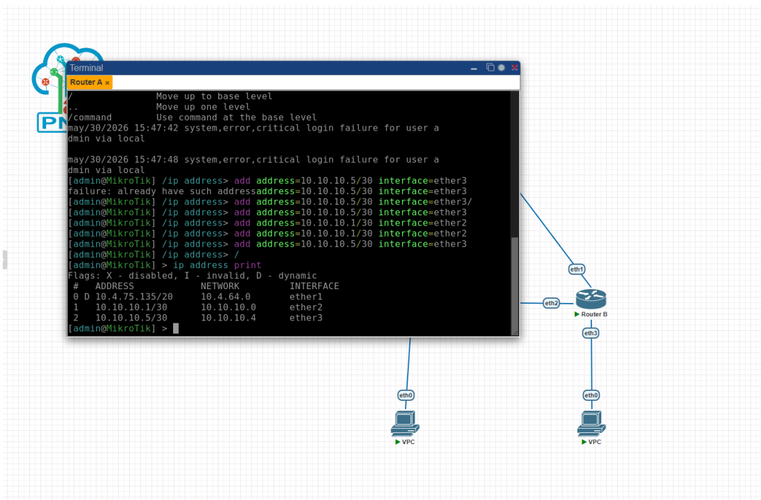
Gambar 3: Hasil Konfigurasi IP Address Router A
